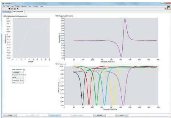
User friendly interface based on LabView
